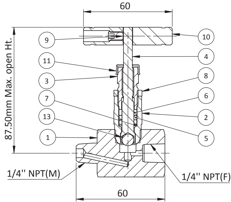
SECTION C-C
