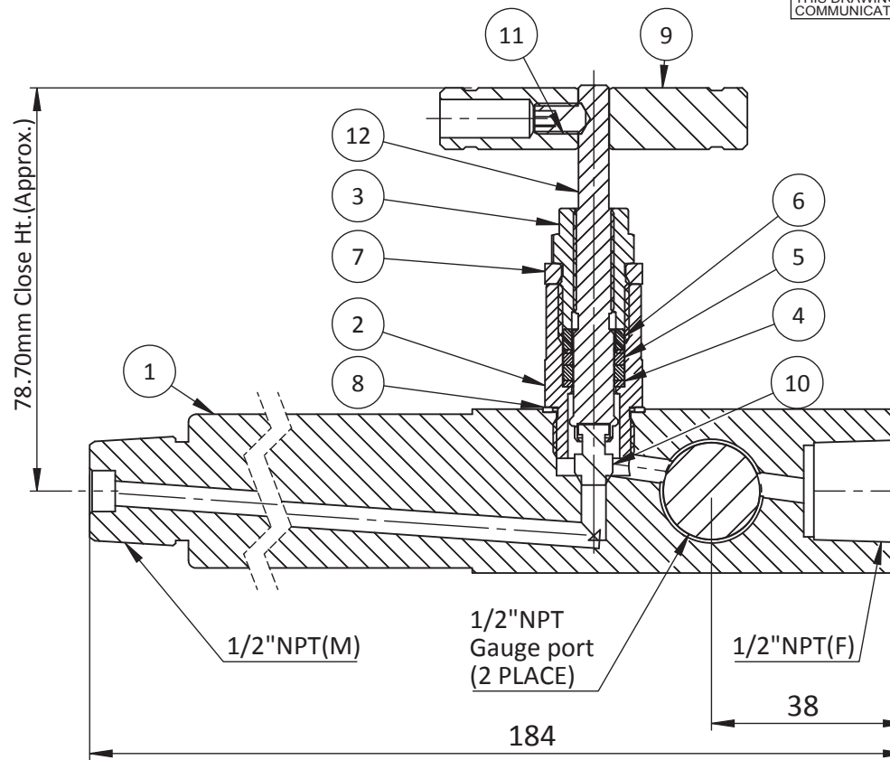
SECTION J-J
